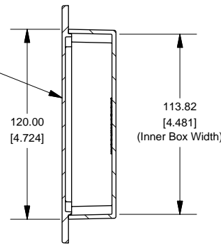
SECTION A-A Side View of Assembly
