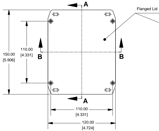
Top View of Assembly
